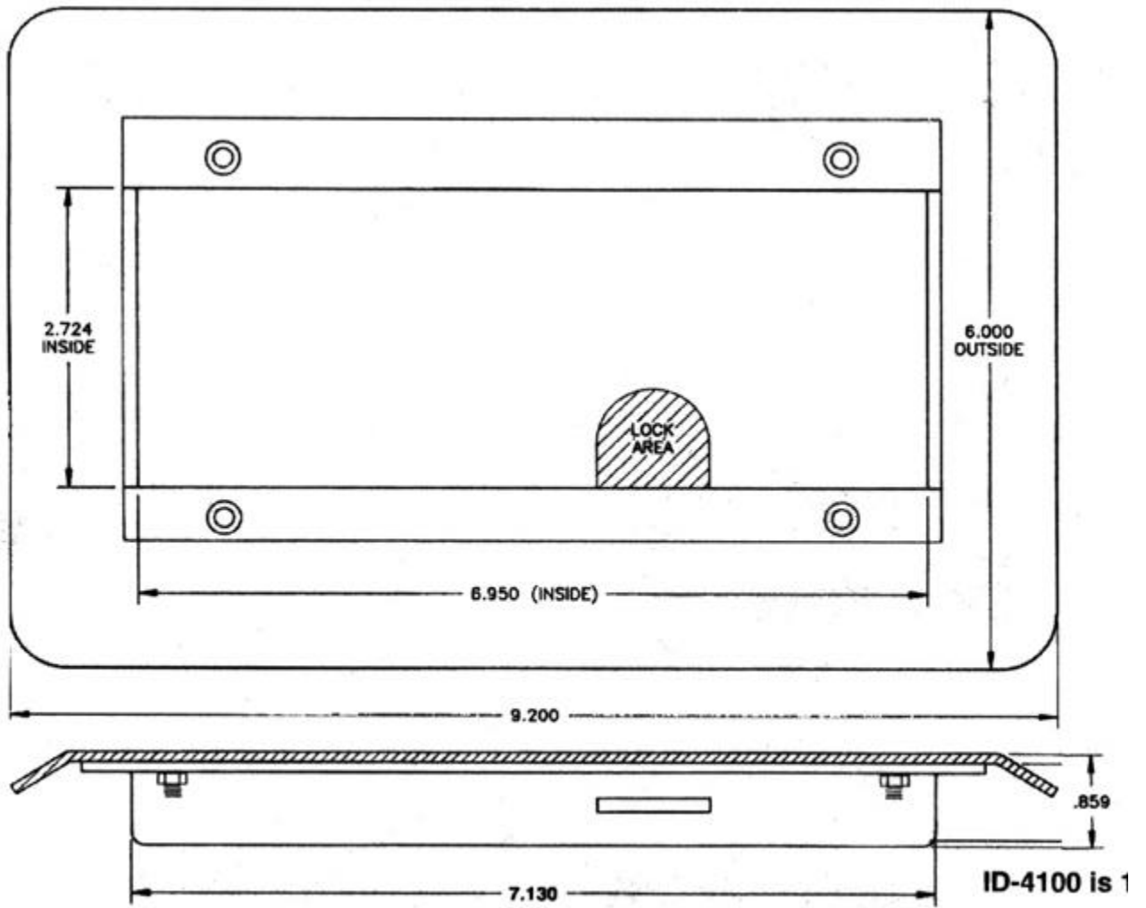
IB-4100/ID-4100 Template
